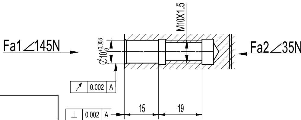
SECTION B-B
